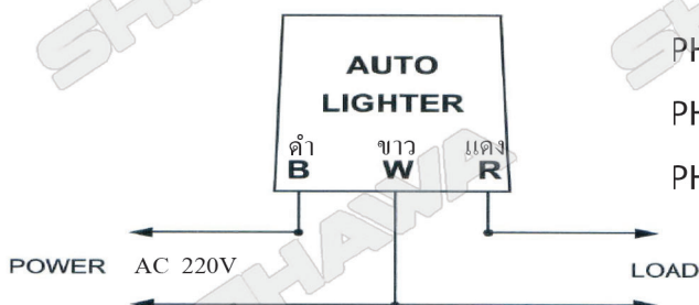
Diagram of Interior Circuit
